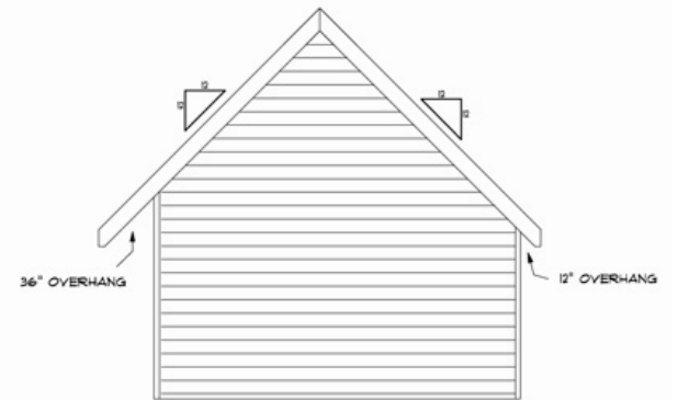
BACK ELEVATION
